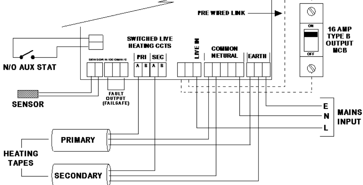
TYPICAL WIRING SCHEMATIC THMU 2
